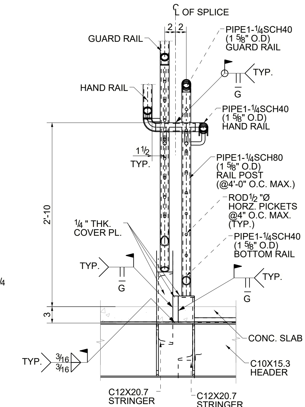
SECTION G1 - G1
