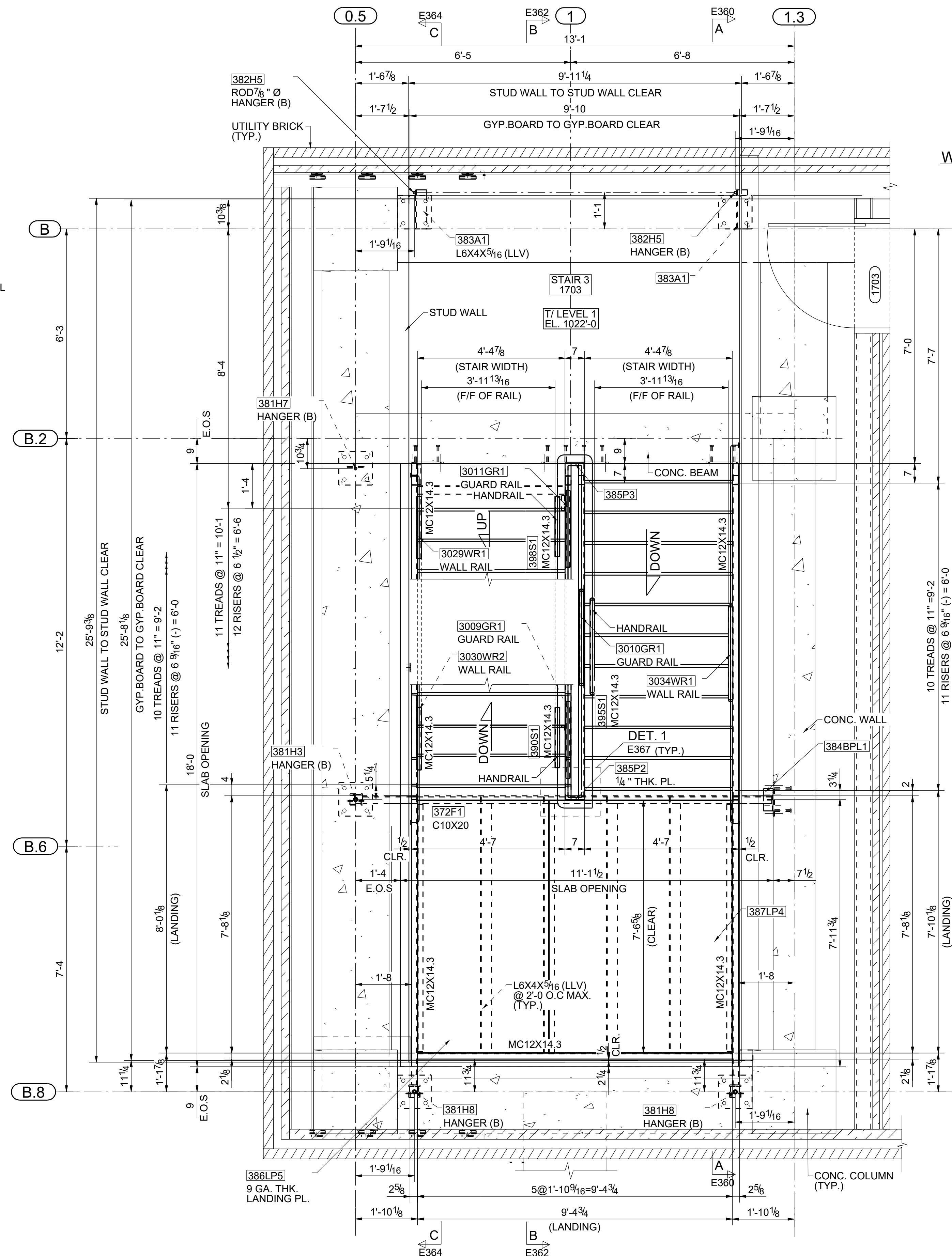
STAIR # 3 PARTIAL FRAMING PLAN @ LEVEL 1 (EL. 1022'-0") (REF: LEVEL 1 - ENLARGED PLAN - STAIR WEST - 1/ A507/ SLAB EDGE - LEVEL 1 - WEST - 1/ S251A)
