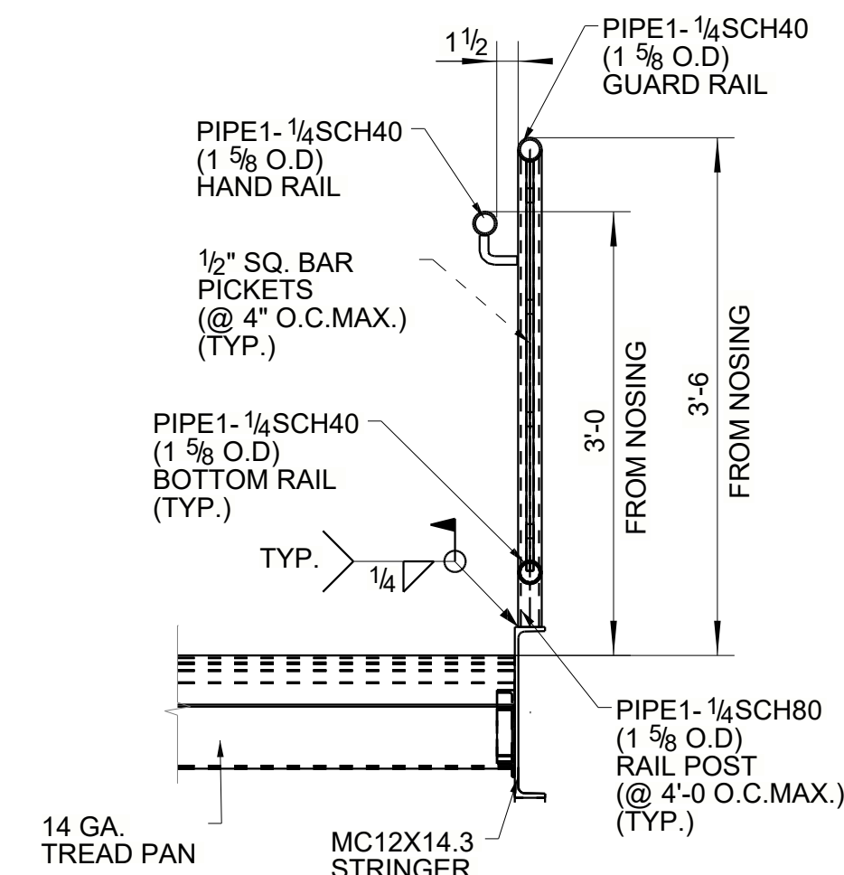
TYPICAL STRINGER RAIL DETAILS
