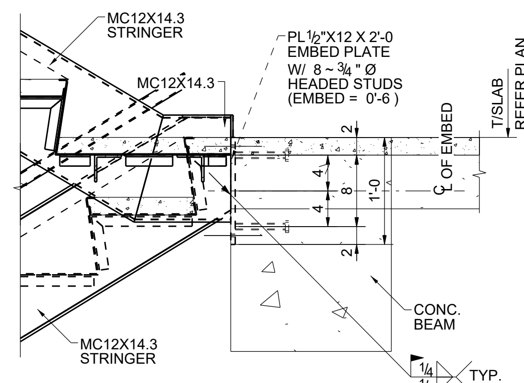
TYPICAL STRINGER TO EMBED CONNECTION DETAILS
