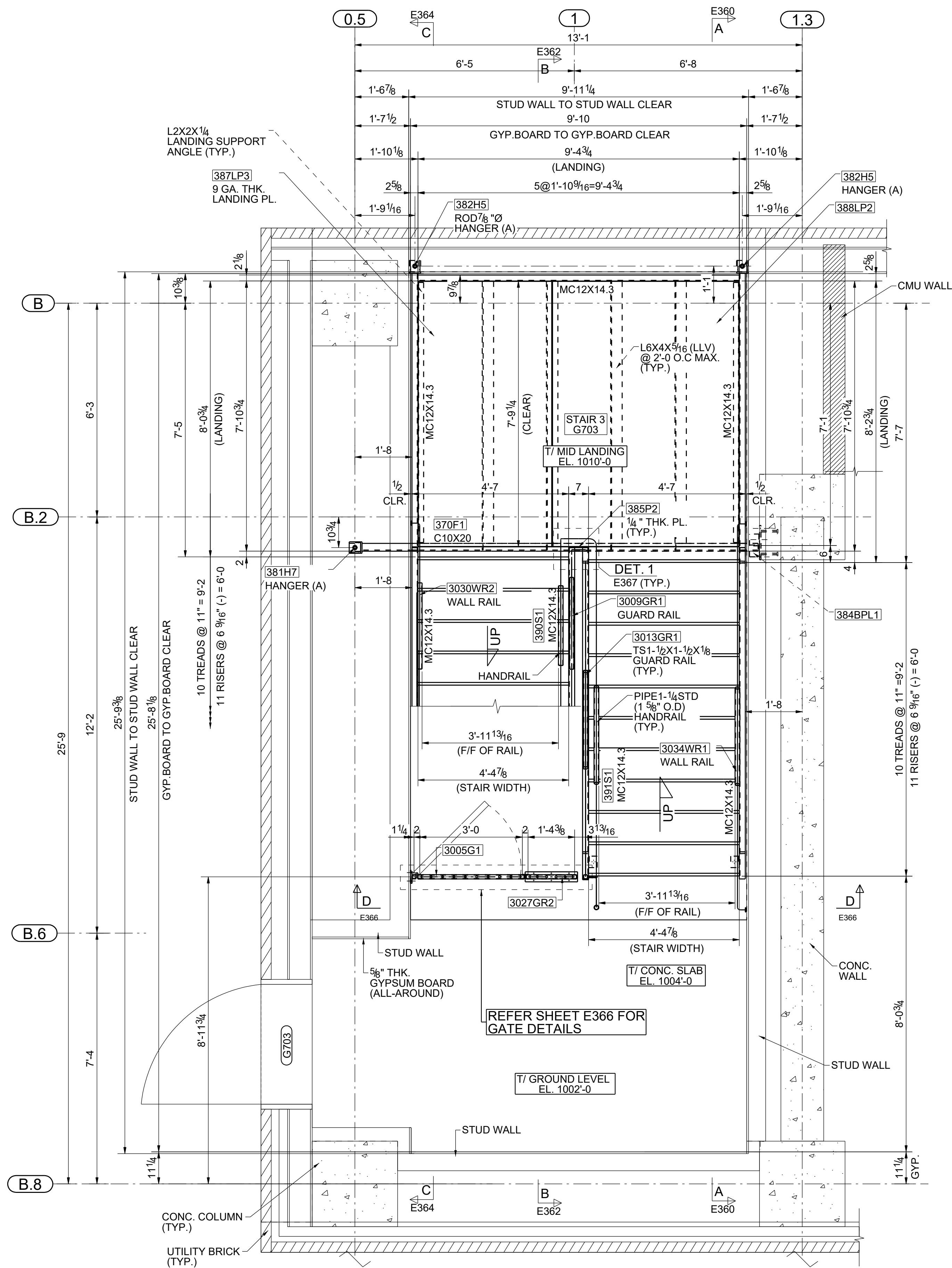
STAIR # 3 PARTIAL FRAMING PLAN @ GROUND LEVEL (T/SLAB AT STAIR LOCATION EL.1004'-0") (REF: GROUND LEVEL - ENLARGED PLAN - STAIR WEST - 0/ A507/ EDGE OF SLAB PLAN - GROUND FLOOR - WEST - 1/ S250A)
