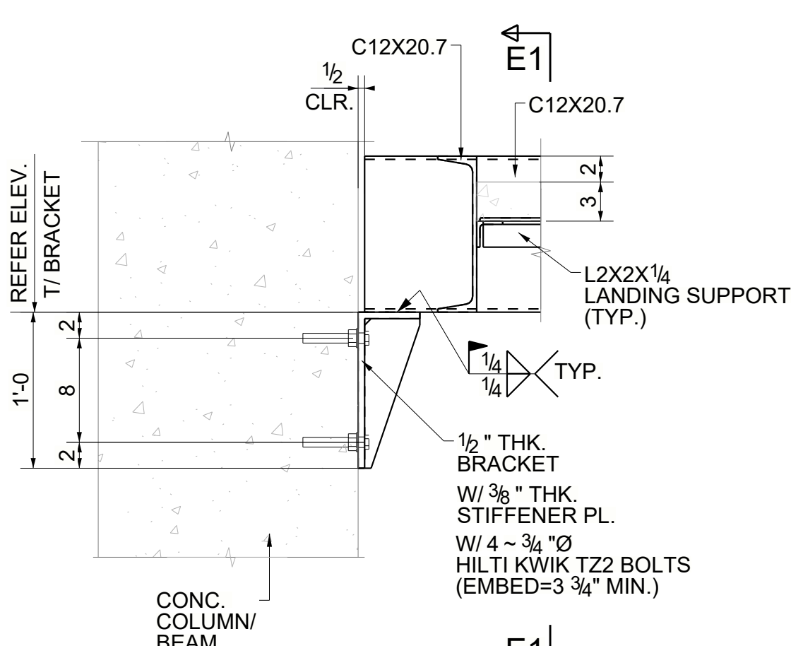
DETAIL E 2-E210
