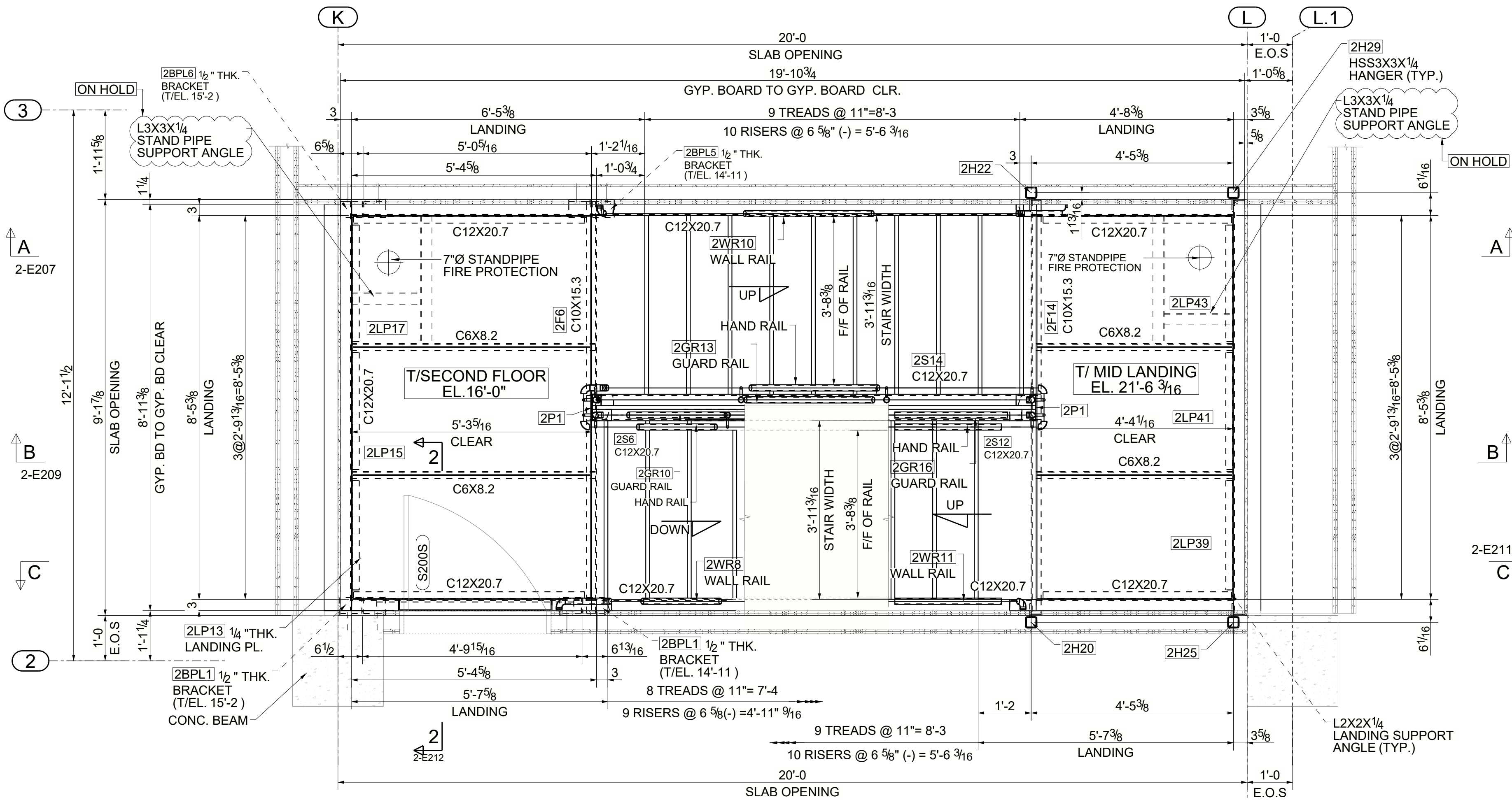
PARTIAL FRAMING PLAN OF SOUTH STAIR @ T/SECOND FLOOR EL. T/ EL. 16'-0
