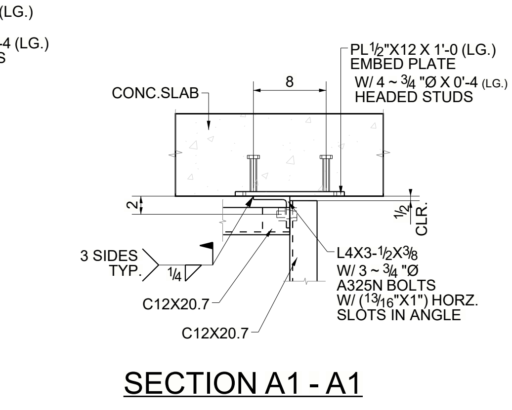
TYPICAL STRINGER RAIL DETAIL (REFER :SECTION AT STRINGER : 17/A403)
