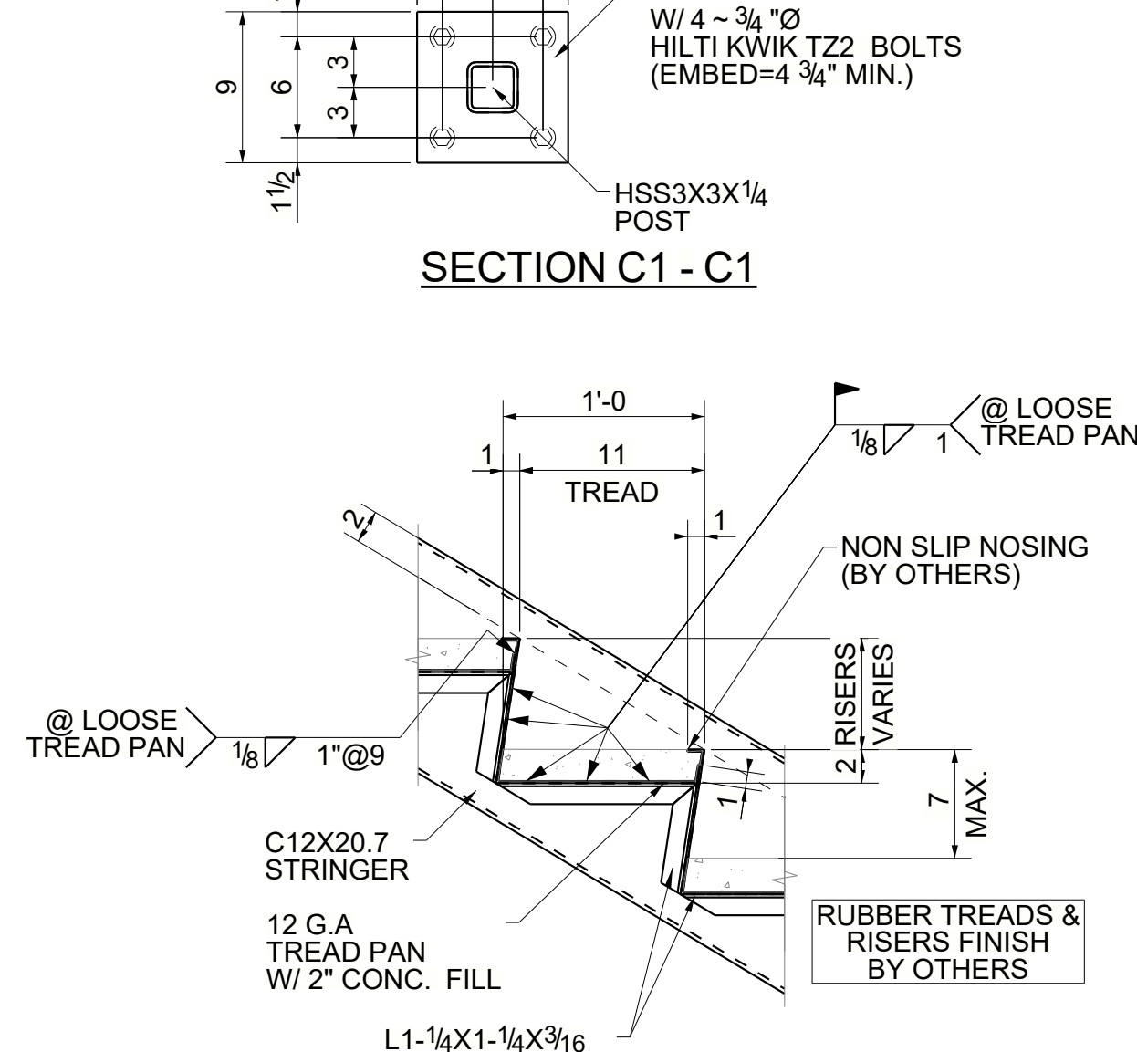
TYPICAL STRINGER TREAD DETAIL
