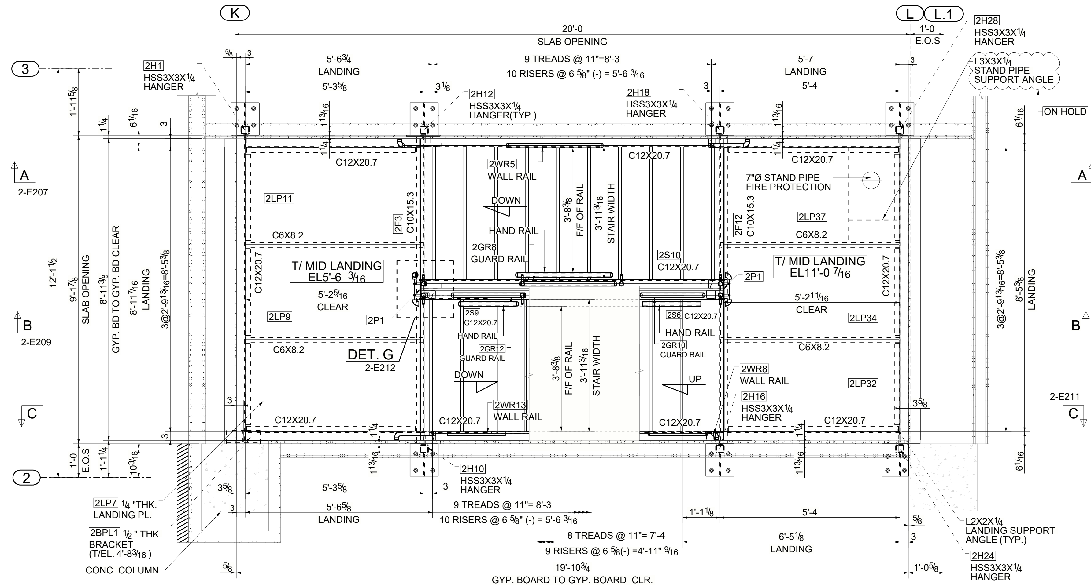
PARTIAL FRAMING PLAN OF SOUTH STAIR @ T/MID LANDING EL. 11'-0 7/16
