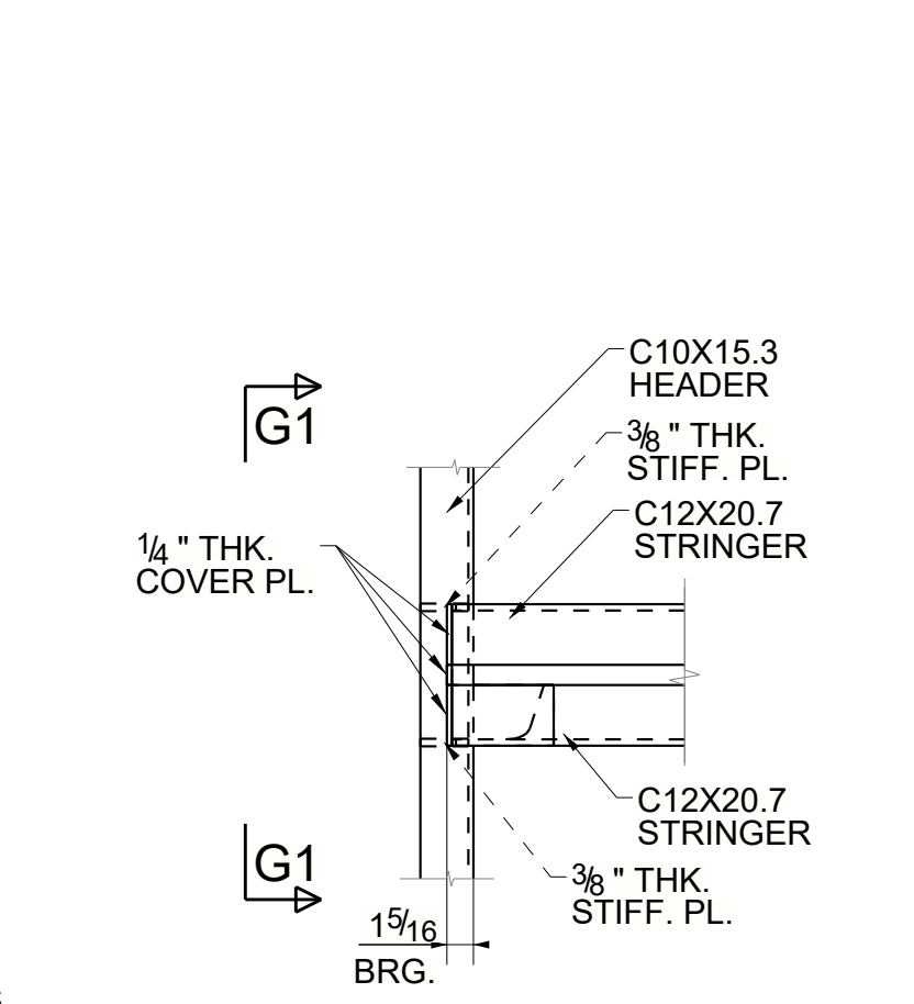
DETAIL G 2-E203
