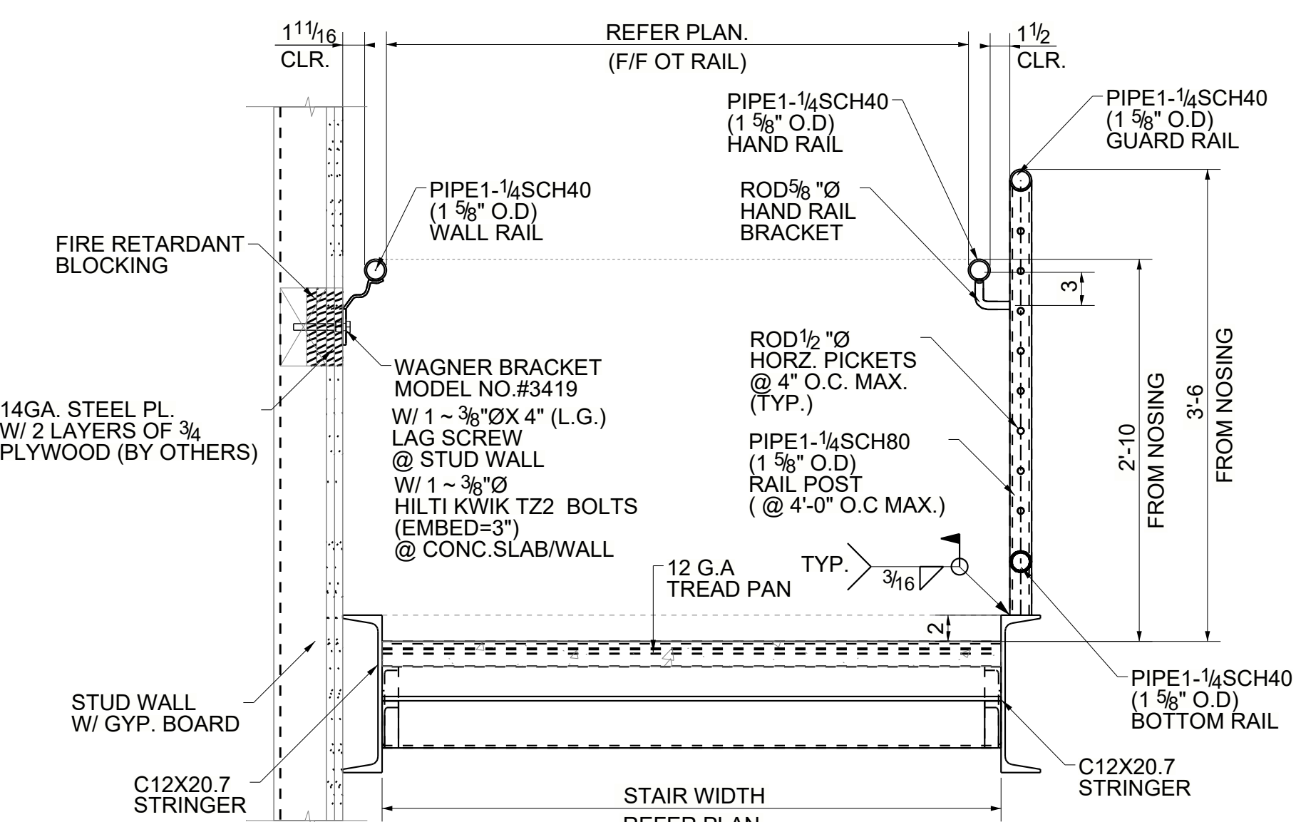
TYPICAL STRINGER RAIL DETAIL (REFER :SECTION AT STRINGER : 17/A403)
